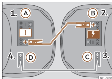
Fig. 176 Jump lead connection diagram.
