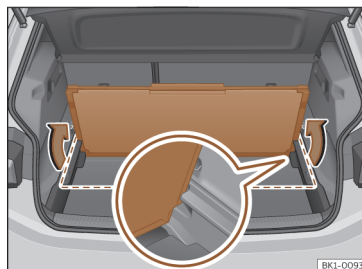
Fig. 165 In the luggage compartment: attach the second luggage compartment floor.
