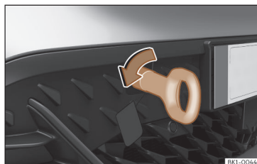
Fig. 178 Right side of the front bumper: towline anchorage screwed in.
