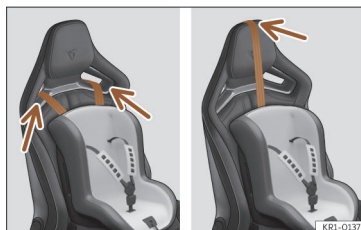
Fig. 43 Front passenger seat: adjustment and assembly according to the Top Tether belt.
