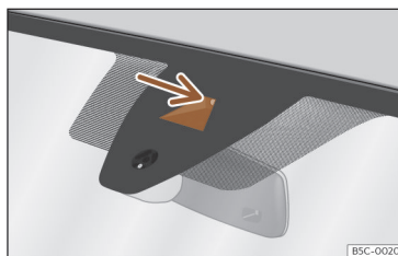
Fig. 111 On the windscreen: field of vision of the Lane Assist system camera.
