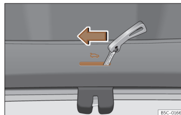
Fig. 79 Luggage compartment: manual release.
